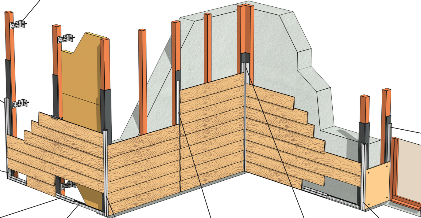
Vis Cédral Board autoforeuse
